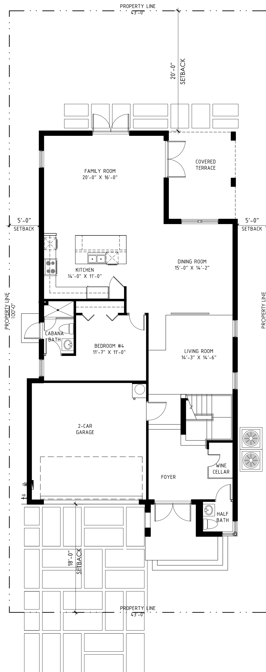
GROUND FLOOR - "B-ALT"
