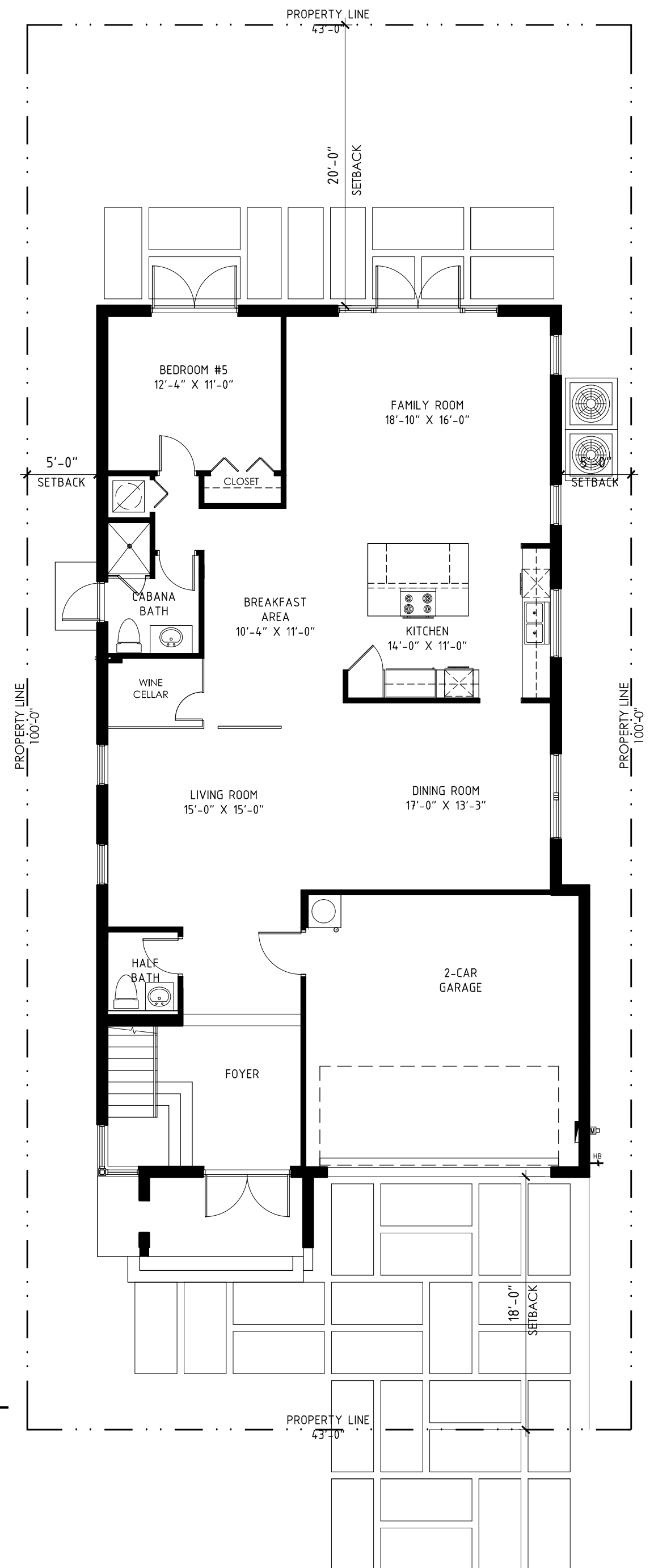
GROUND FLOOR - "C-ALT"
